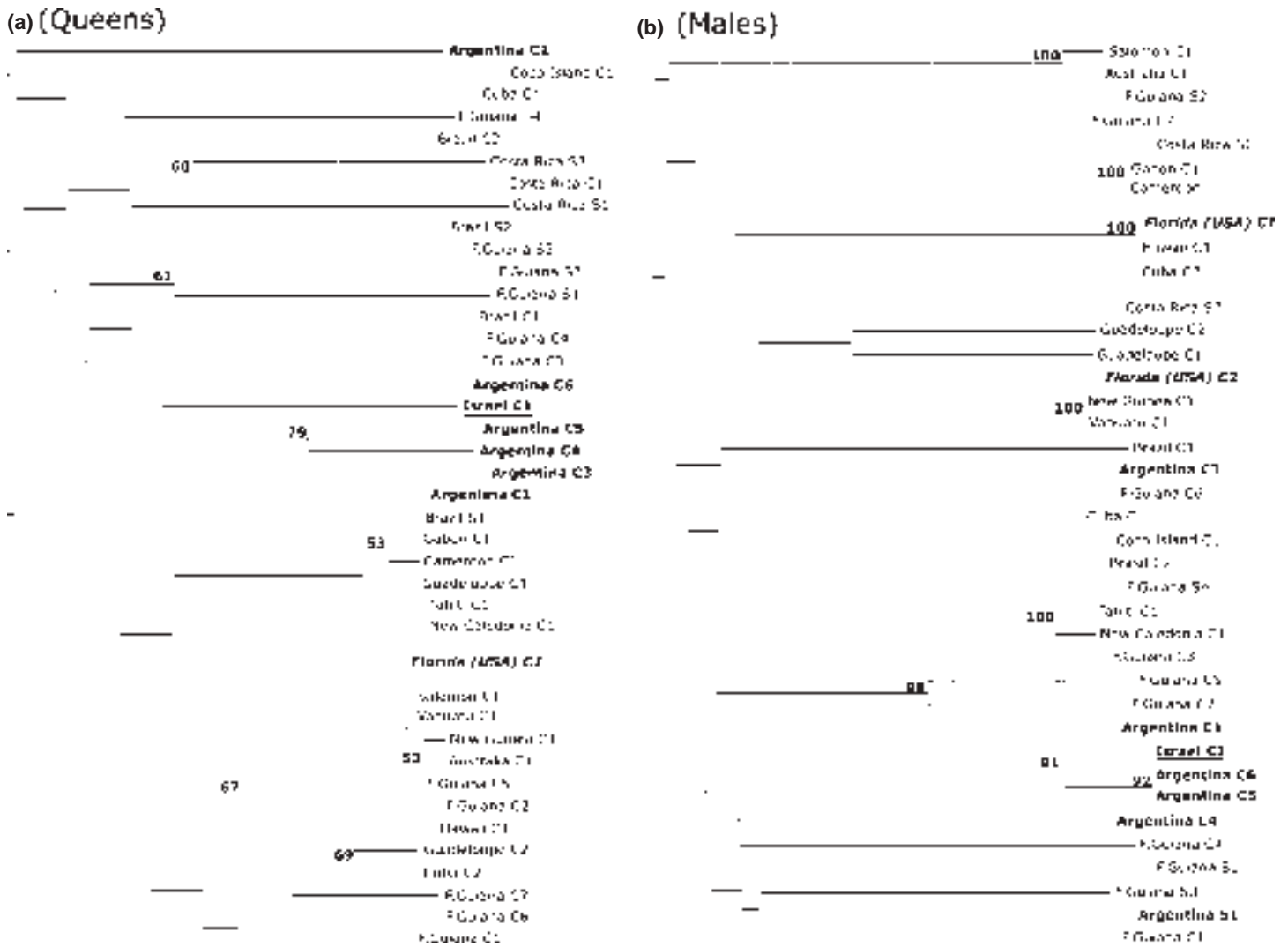
Figure 3 NJ dendrograms of the microsatellite allele shared distances between individual queens (a) and males (b). The Argentinean genotypes are shown in bold characters, the Florida genotypes are shown in bold italic characters and the Israeli genotype is shown in underlined bold characters. Dendrograms are not rooted, due to the lack of PCR amplification for many W. auropunctata microsatellite loci in the closely related species W. rochai used as an outgroup in Fig. 2. Bootstrap values (computed from 1000 replicates) for nodes are shown only when > 50%. Note that low bootstrap values (bootstrapping over loci) are usually obtained for trees with individuals as tips.
