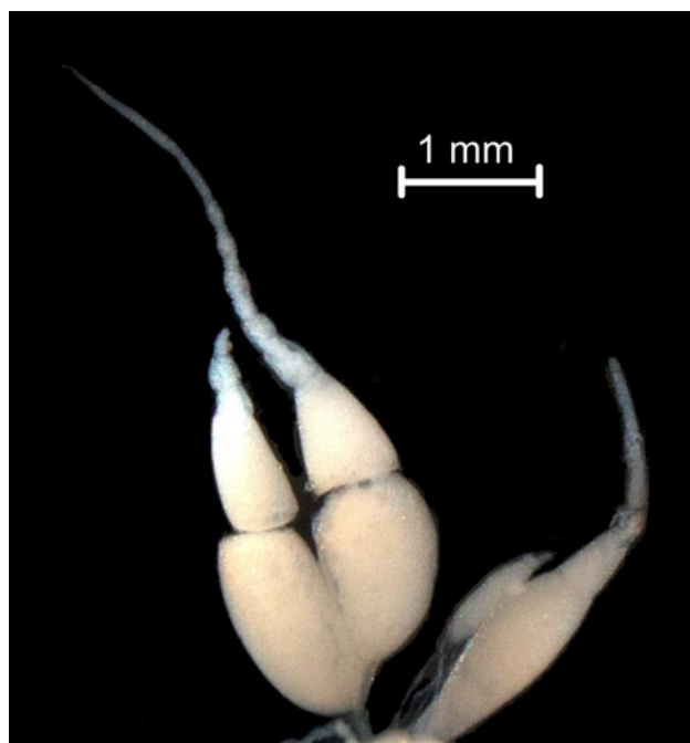
Fig. 4 Gaster dissection of A. gracilipes worker, showing ovarioles with no evidence of yolky oocyte development or yellow bodies
